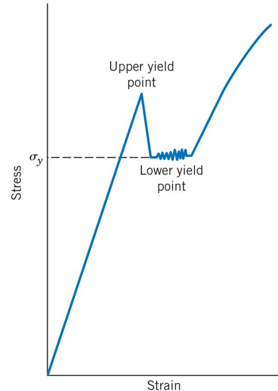
Yield point phenomenon
